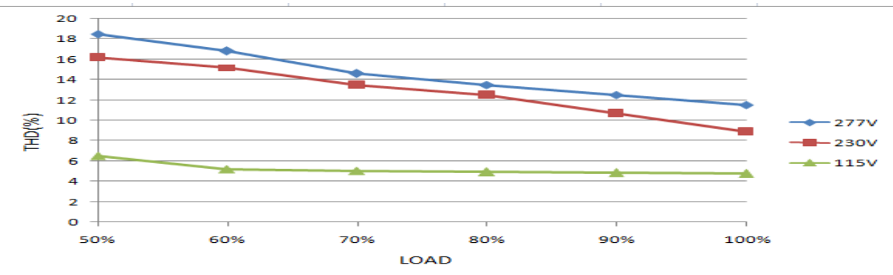
THD vs LOAD
