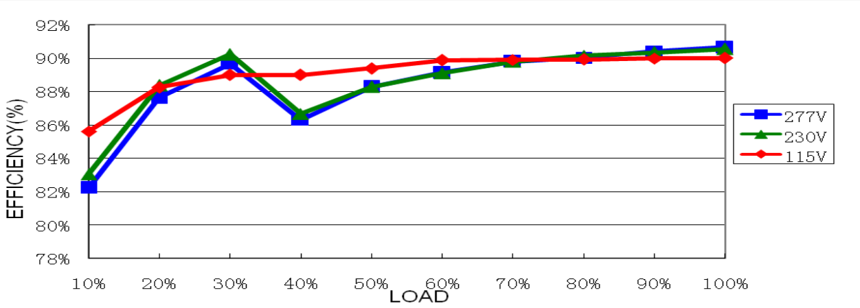
EFFICIENCY vs LOAD
