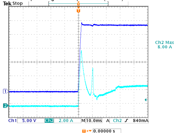
INPUT=24VDC @ FULL LOAD
